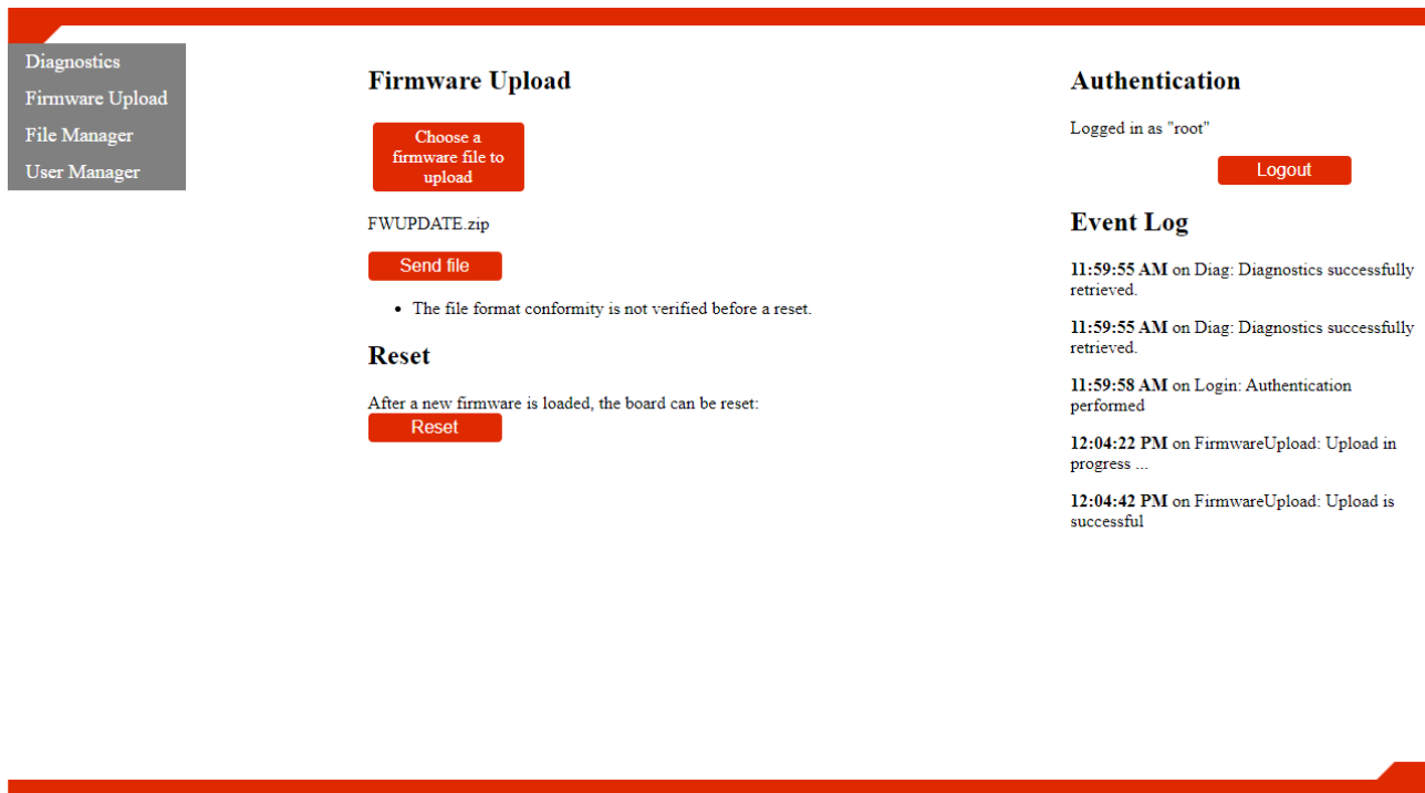
Figure 5: Firmware upload
