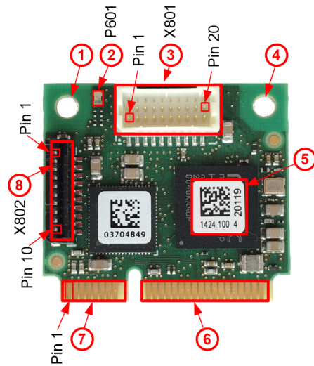
Figure 1: Basic card CIFX HPCIIE90 (Revision 4)
