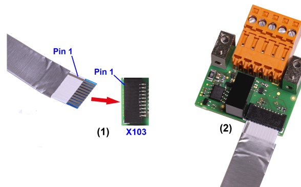
Figure 5: Plug the cable into the cable connector fieldbus X103 on the AIFX-V2-DN
